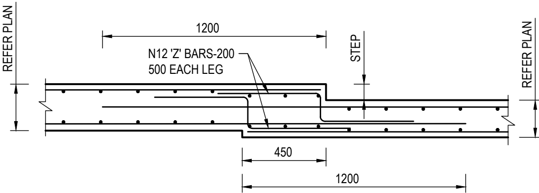
TYPICAL FOLD/STEP DETAIL SCALE 1:20
