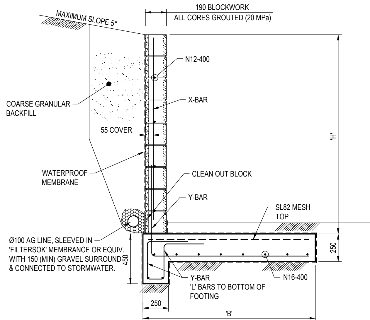
TYPICAL BLOCK RETAINING WALL DETAIL RW1
