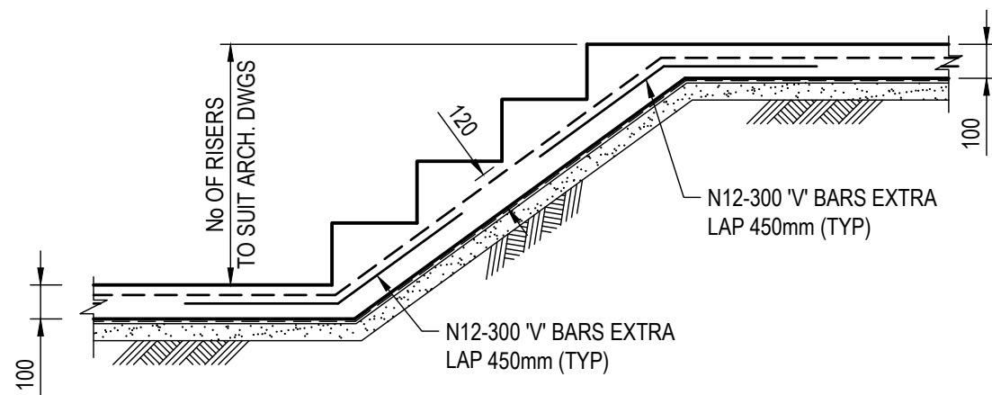
TYPICAL WALKWAY STAIRS
