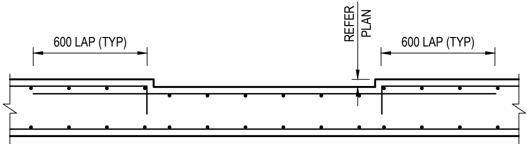
TYPICAL WET AREA SETDOWN DETAIL SCALE 1:20
