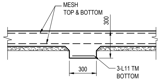
TYPICAL 'IB1' DETAIL
