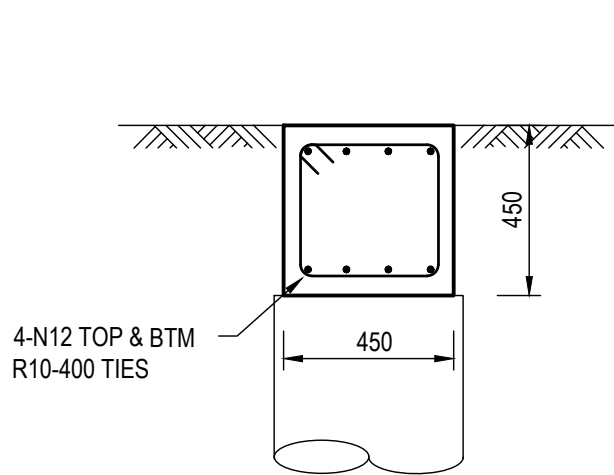
TYPICAL 'SF1' DETAIL
