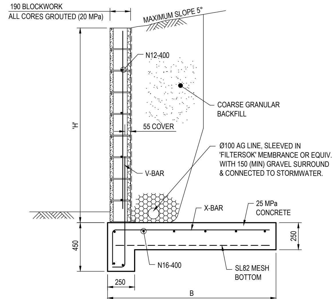
ALTERNATE BLOCK RETAINING WALL DETAIL 'RW1'
